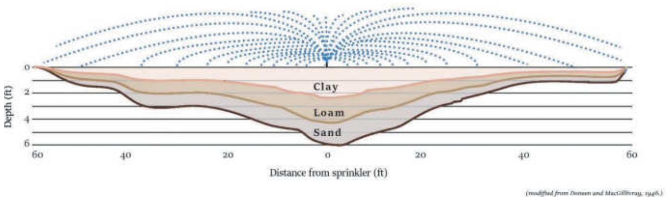
Figure 26. Depth of applied water in the soil by a single sprinkler, based on different soil textures with a single application rate. As the distance from the sprinkler increases, the application of water from a sprinkler decreases. Higher application rates of applied water lead to greater differences in penetration depth of soil moisture. A well-designed sprinkler system spaces sprinkler heads in a manner that achieves overlap to attain maximum uniformity. (Drawing by Nancy Villeda.)
