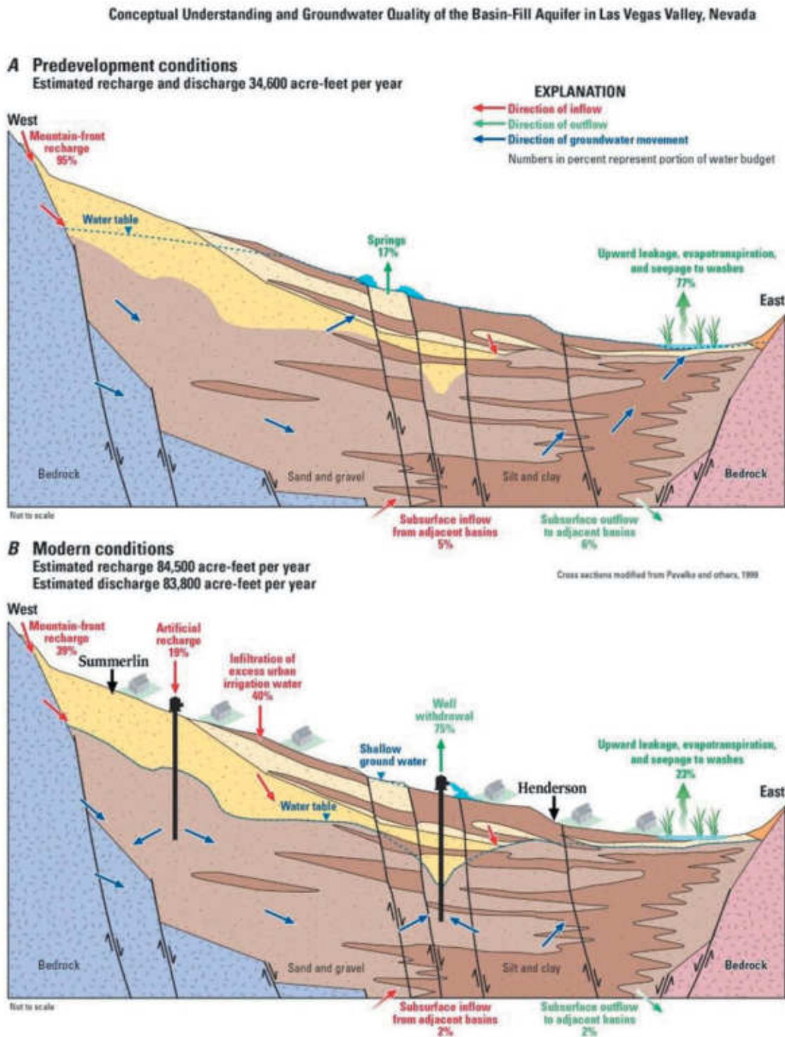
Figure 3. Generalized cross-sections for Las Vegas Valley, Nevada, showing the basin-fill deposits and components of the groundwater flow system under (A) predevelopment conditions and (B) modern conditions.
